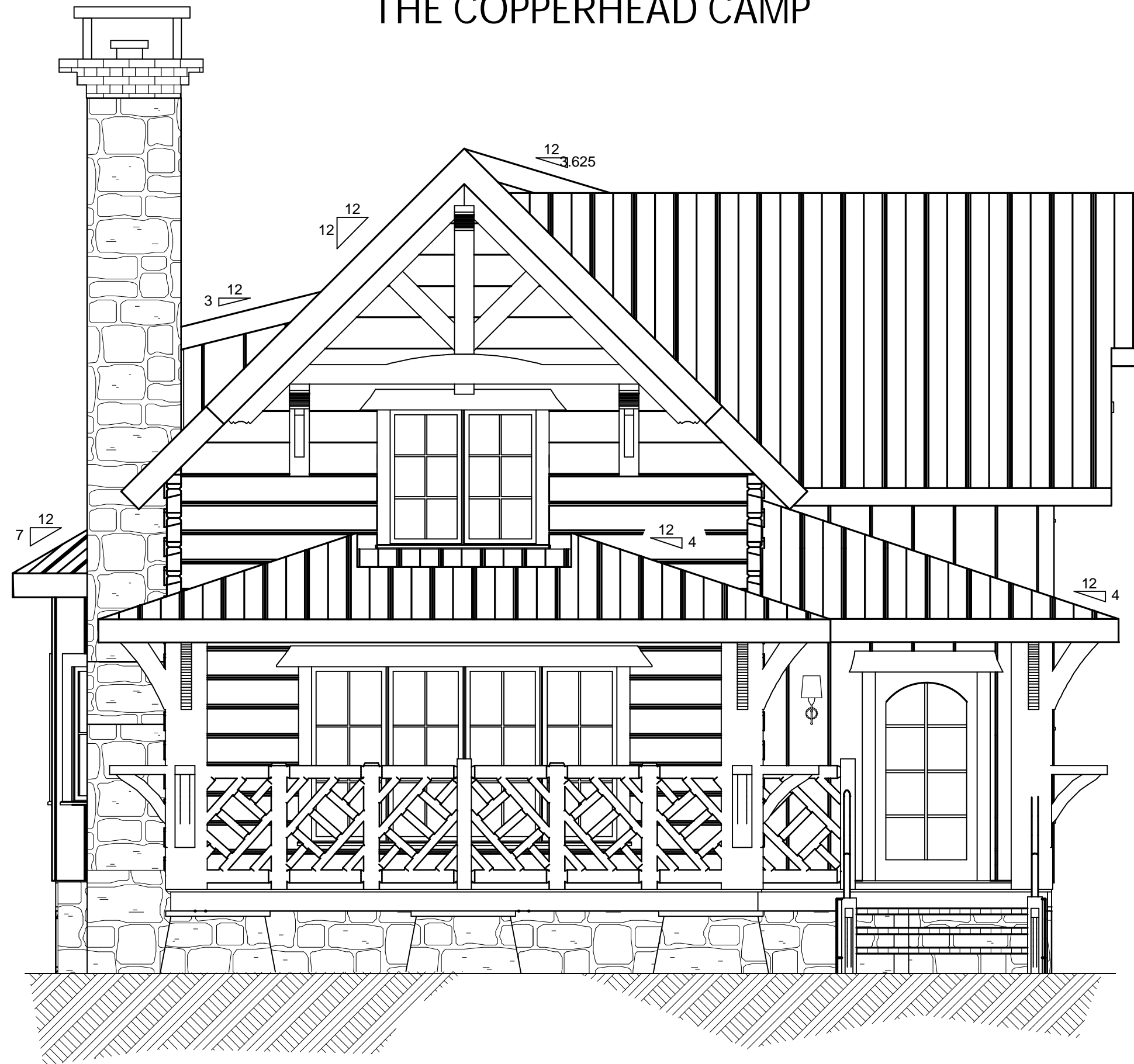
FRONT ELEVATION
